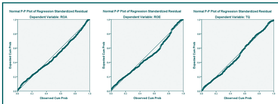
Figure 3 Results of P-P plot
